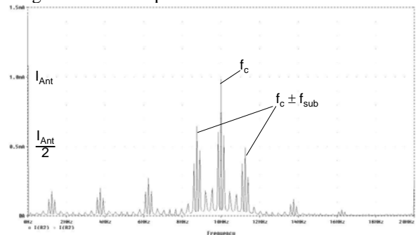
Figure 14 shows the frequency spectrum of the output signal of the simple ring modulator in an endless sequence of 1-bits
