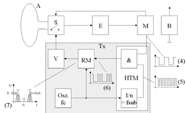
Figure 4: Basic circuit of a transponder, generating active load modulation.
