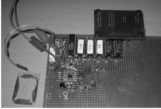
Figure 12: A first setup to generate active load modulation for ISO/IEC 14443. The smart card chip is placed on the small board connected on the top.
