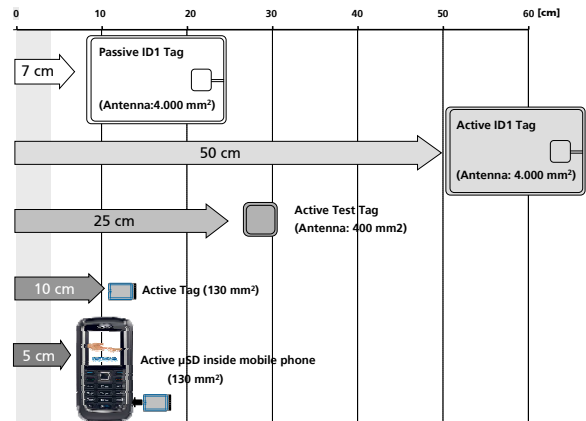
Figure 7 shows the difference in the ranges of active and passive systems with different antenna sizes.
