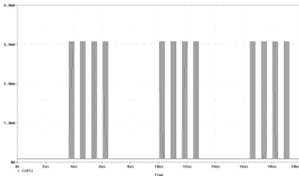
Figure 16 shows the output of the ASK modulator with an endless sequence of 1-bits in the time domain.
