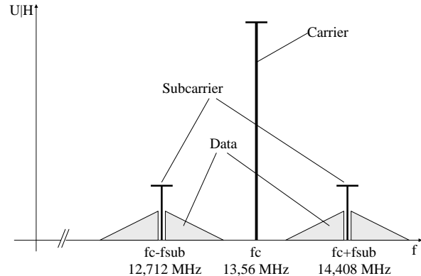
Figure 3 shows the frequency spectrum at the reader antenna resulting from a common passive load modulation with a subcarrier, according to ISO/IEC 14443-2.
