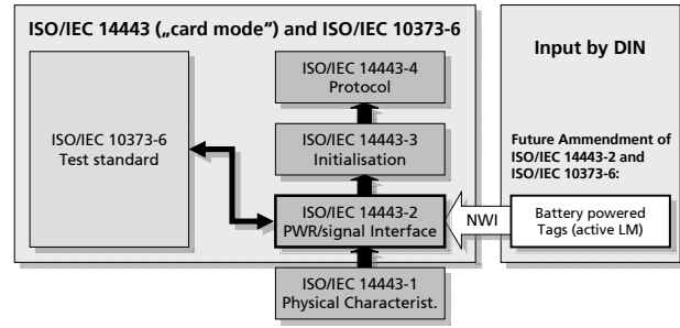
Figure 19: Our approach of standardising active load modulation in ISO/IEC 14443
