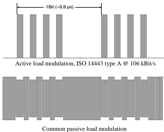
Figure 6 shows the RF Signal at 13.56 MHz of an active and a passive transponder, while transmitting the same data signal.
