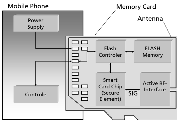
Figure 9 Components of a secure micro SD card with an active RFID interface.
