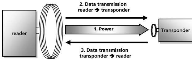
Figure 2: The limiting factors of a contactless communication. (1) Power transfer: the small antenna cannot extract enough power from the field and therefore (2) not receive any data. (3) Load modulation: the return signal from the small antenna to the reader is too small with load modulation
