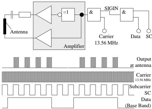
Figure 5 shows an ASK modulator to generate an ASK type active load modulation.
