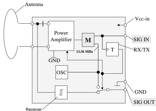
Figure 11 shows a simplified block diagram of the required active RFID interface module.
