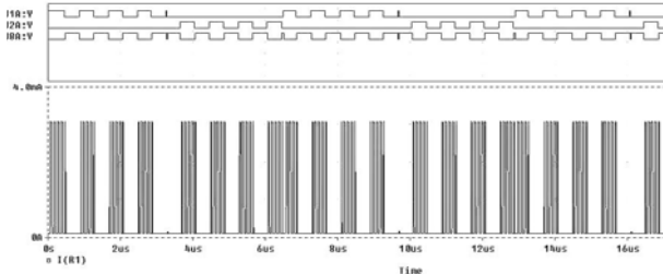
Figure 18: Output signal of an ASK modulator, using a BPSK modulated load modulation subcarrier.
