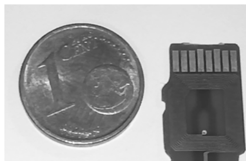
Figure 8: Size comparison –micro-SD sized transponder antenna
