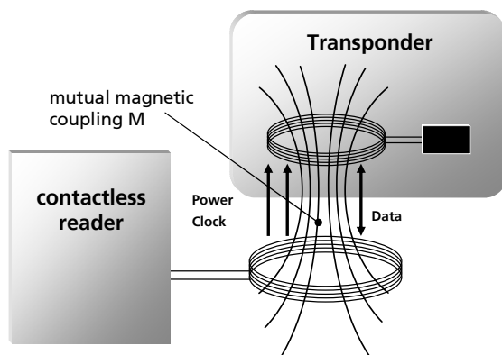
Figure 1: An inductive coupled RFID system uses mutual magnetic coupling to transfer power and data.
