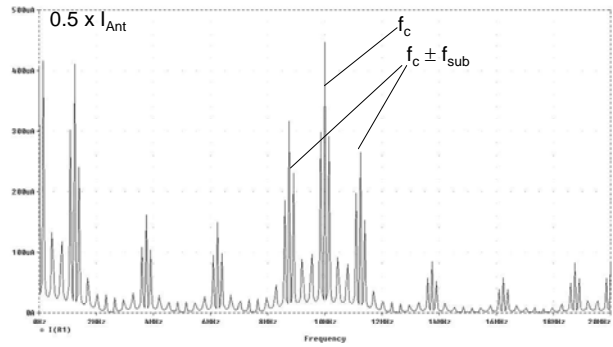
Figure 17 shows the frequency spectrum of the output signal of the ASK modulator with an endless sequence of 1-bits.
