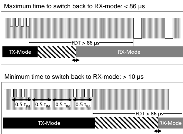
Figure 13 shows the minimum and maximum hold times of the timing element defined by the FDT (top) and the bit interval at 106 kbit/s (bottom).
